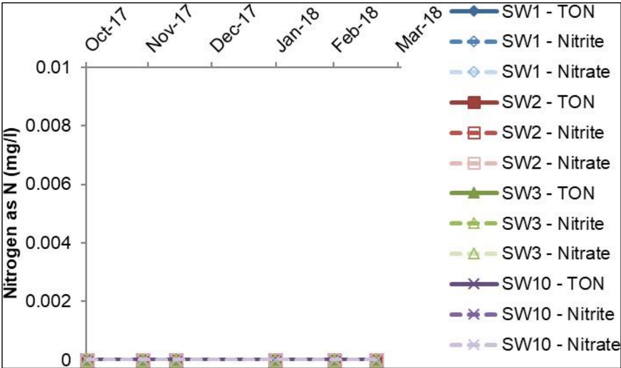
Figure 2 – Surface water Nitrate levels at Abbots Moss Site 1-3 and 10 (outflow)
